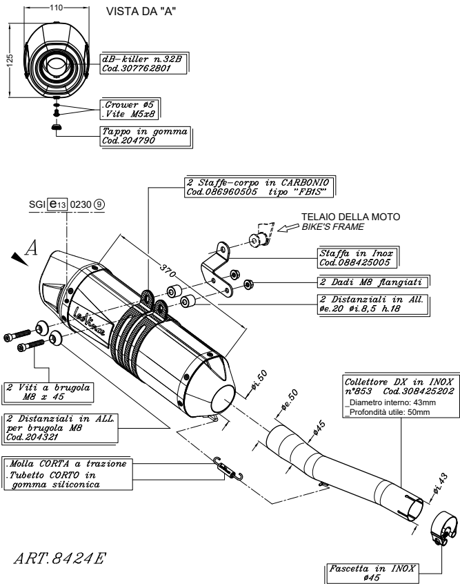
HONDA XRV 750 AFRICA TWIN
