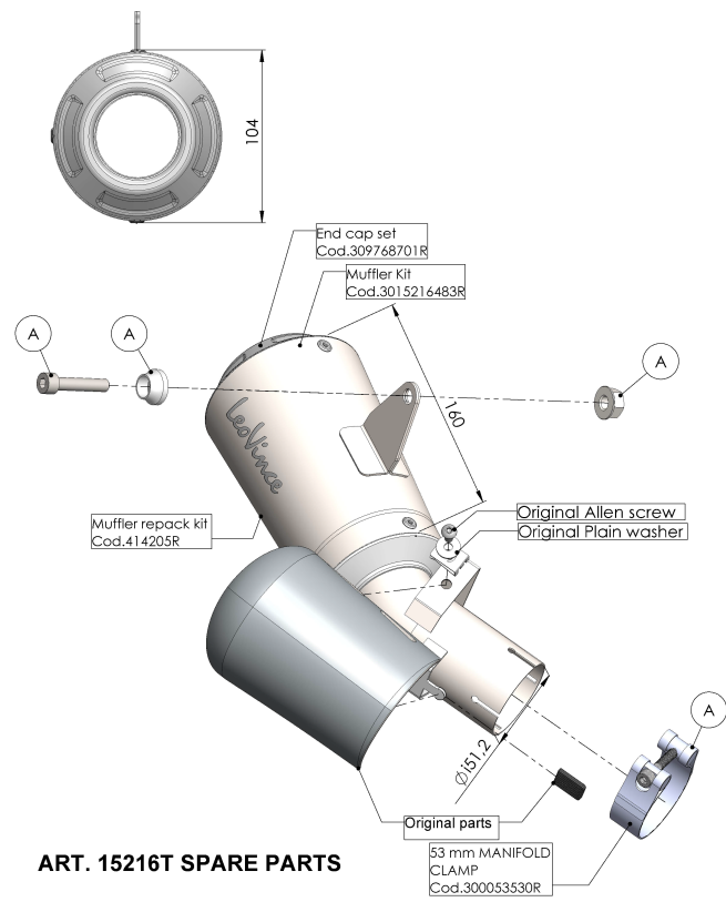
ART. 15216T SPARE PARTS
