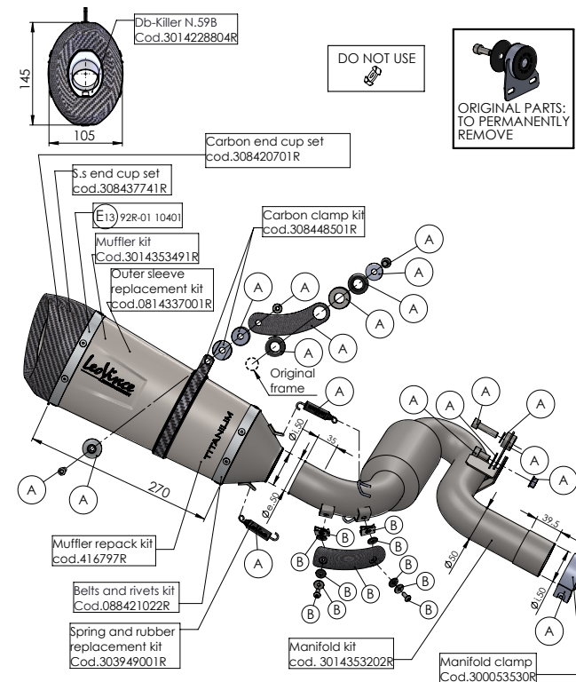
ART. 14353ST SPARE PARTS
