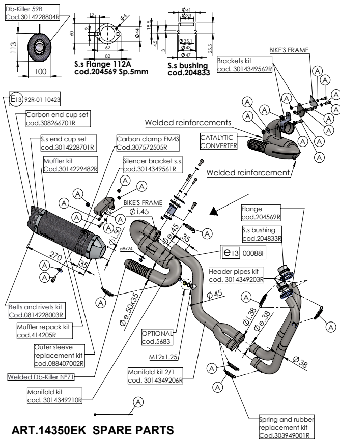
ART.14350EK SPARE PARTS
