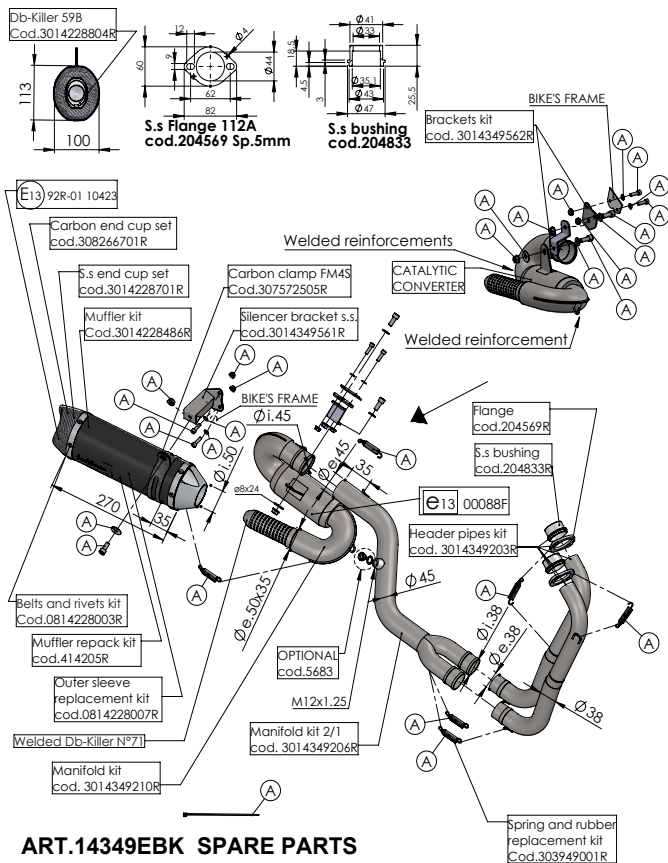
ART.14349EBK SPARE PARTS
