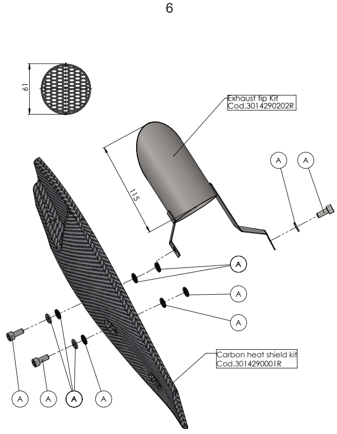
ART. 14290 SPARE PARTS
