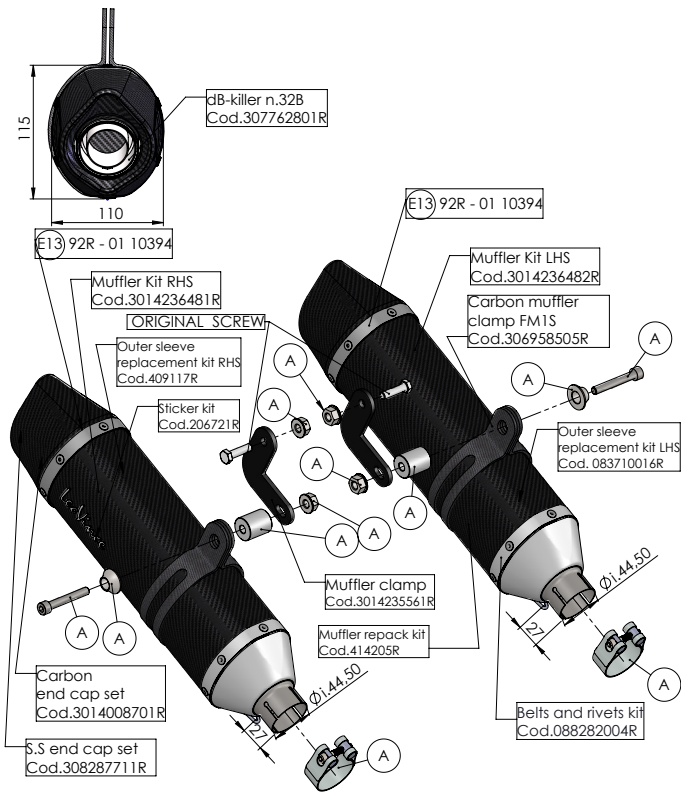
ART. 14236E SPARE PARTS
